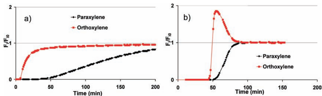
Figure 9. Breakthrough curves of the OX/PX mixture on (a) ZIF-8 and (b) zeolite \beta at 398 K. P(OX) = 320 Pa, P(PX) = 260 Pa.
