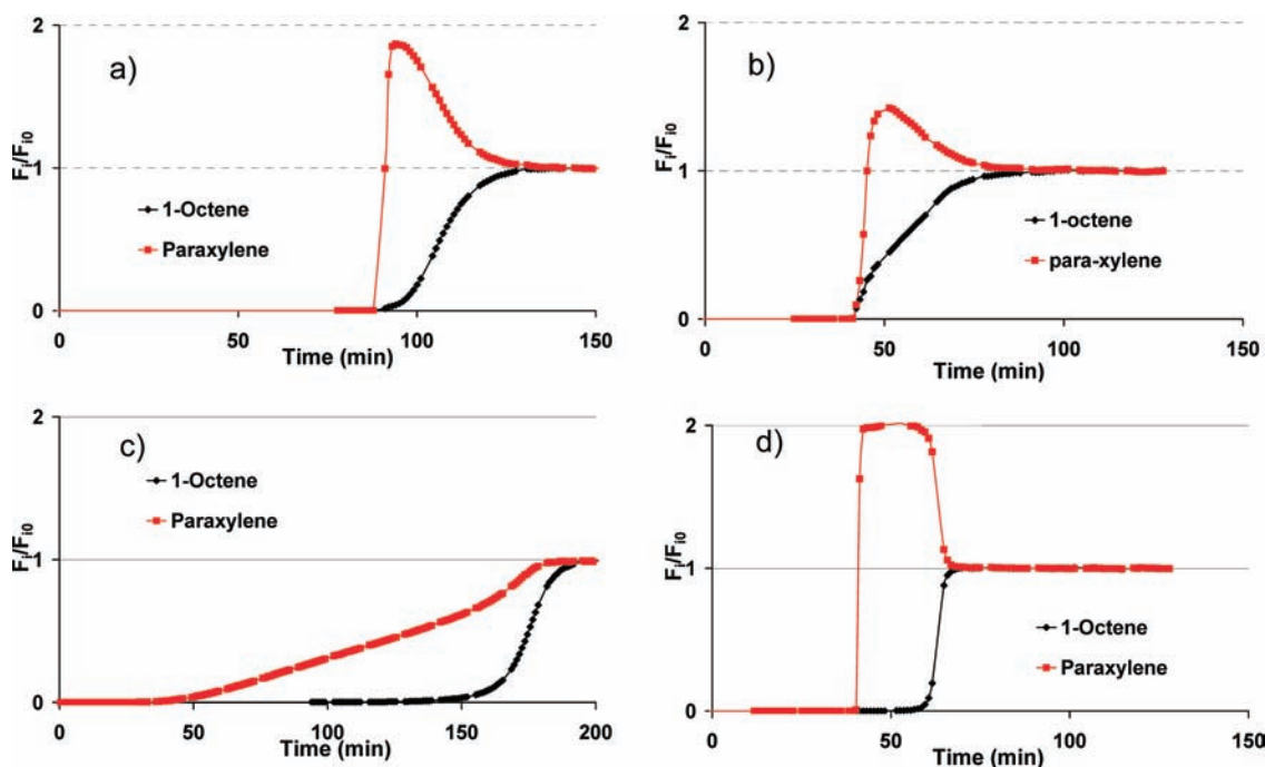
Figure 7. Breakthrough curves of the 1-octene/PX mixture on (a) HKUST-1, (b) CPO-27-Ni, (c) ZIF-8, and (d) zeolite \beta at 398 K. P(=C8) = 300 Pa, P(PX) = 380 Pa.
