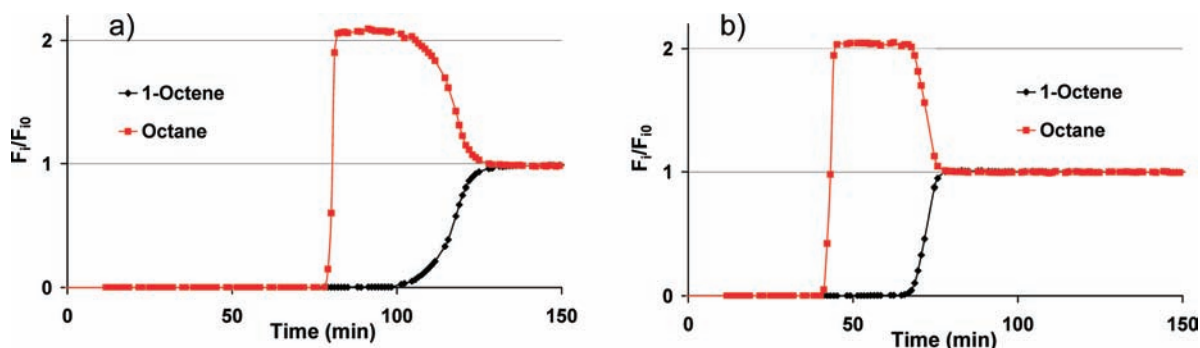
Figure 2. Breakthrough curves of the 1-octene/ n -octane mixture on (a) HKUST-1 and (b) NaY at 398 K. P(=C8) = 600 Pa; P(nC8) = 470 Pa.
