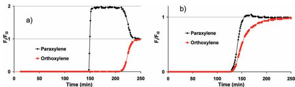
Figure 8. Breakthrough curves of the OX/PX mixture on (a) CPO-27-Ni and (b) ZIF-76 at 398 K. P(OX) = 320 Pa, P(PX) = 280 Pa.
